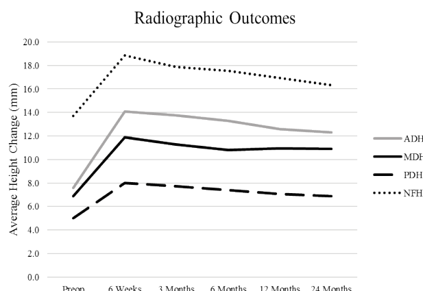
Figure 3: Mean radiographic measurements are shown. The results showed a significant increase from baseline for each parameter and sustained at 3, 6, 12, and 24 months (ADH=Anterior Disc Height; MDH=Middle Disc Height; PDH=Posterior Disc Height; NFH=Neuroforaminal Height).
